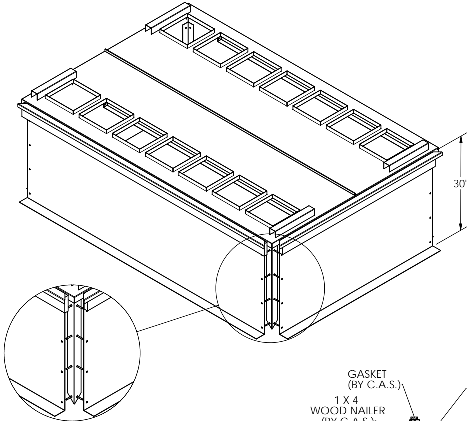
DETAIL A
